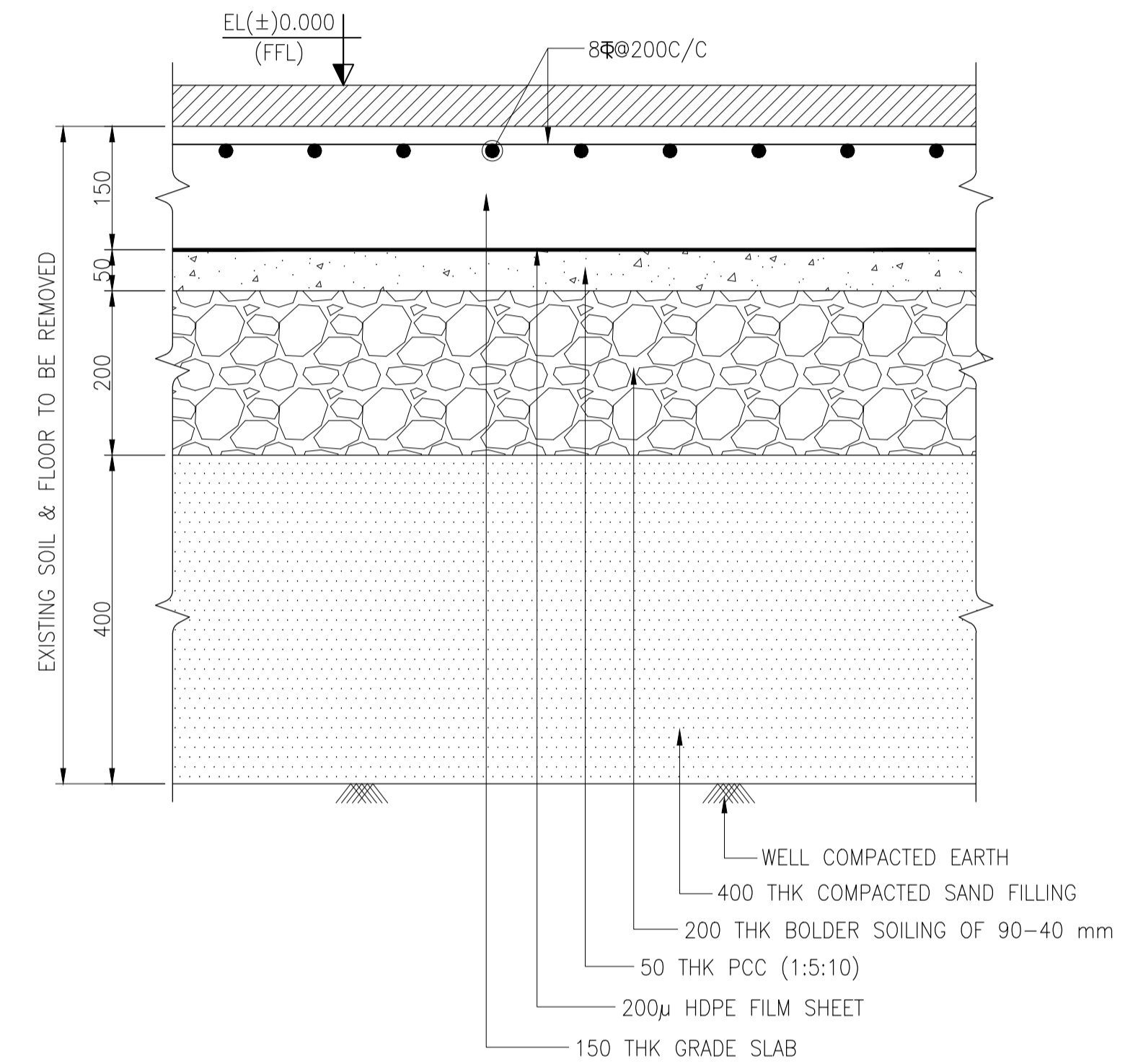
FLOOR OF REBUILT TYPICAL SECTION FOR DAMAGED FLOOR
