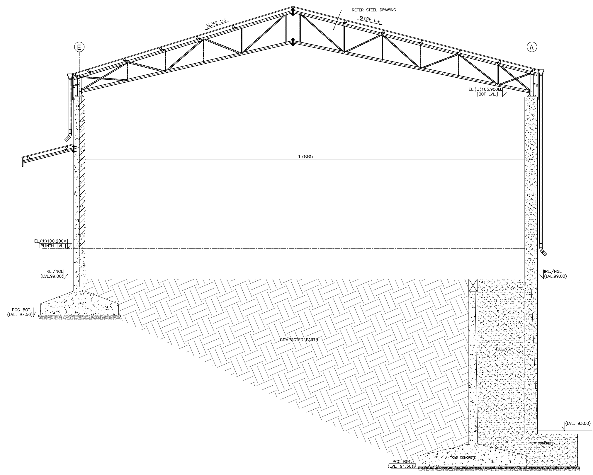
TYPICAL SECTION
